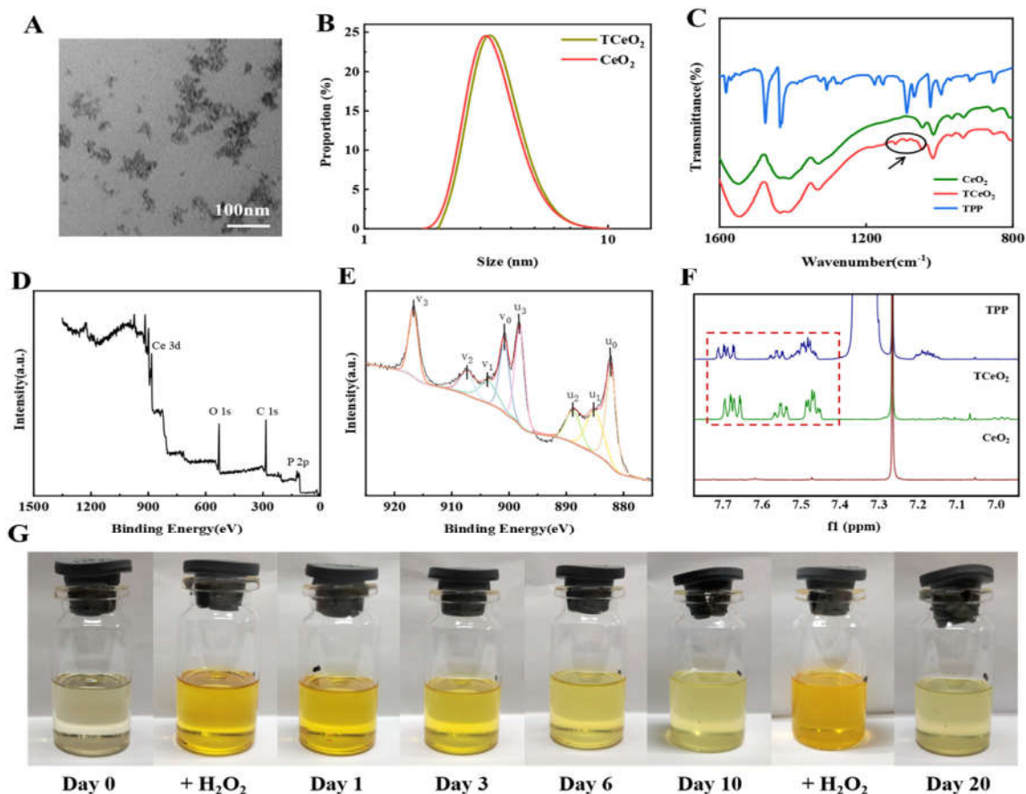
Fig.1. Characterization of TCeO 2 . (A-B) TEM image of TCeO 2 , DLS results of TCeO 2 and CeO 2 ; (C) Infrared spectra of CeO 2 , TCeO 2 and TPP; (D) XPS spectrum of TCeO 2 ; (E) Ce 3d XPS spectrum of TCeO 2 ( u_0=882.20 eV, u_1=885.03 eV, u_2=888.78 eV, u_3=898.11 eV; v_0=900.80 eV, v_1=903.63 eV, v_2=907.38 eV, v_3=916.71 eV); (F) 1 H NMR spectra of TPP, TCeO 2 , and CeO 2 (in CDCl 3 ); (G) The valence cycling ability of TCeO 2 .
